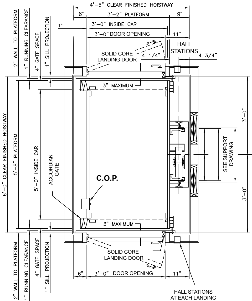
TYPICAL 3' X 5' R/H SAME SWING OPPOSITE HANED LANDING DOORS
