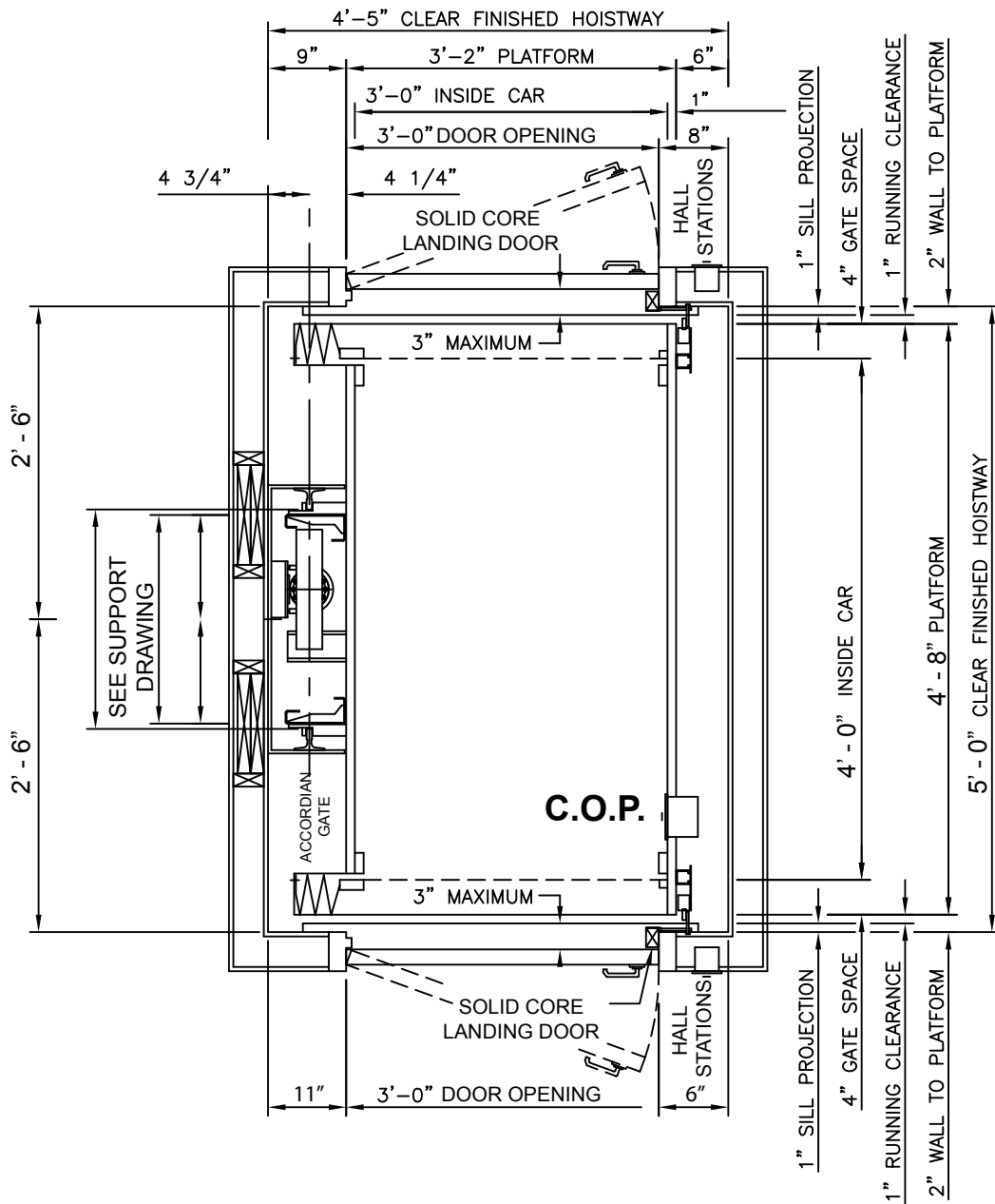
TYPICAL 3' X 4' L/H WITH R/H SAME SWING DOORS
