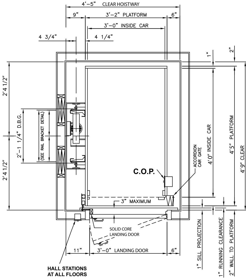
TYPICAL 3' X 4' L/H WITH LEFT HAND LANDING DOORS
